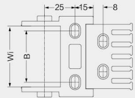
活动端 Moving Bracket
